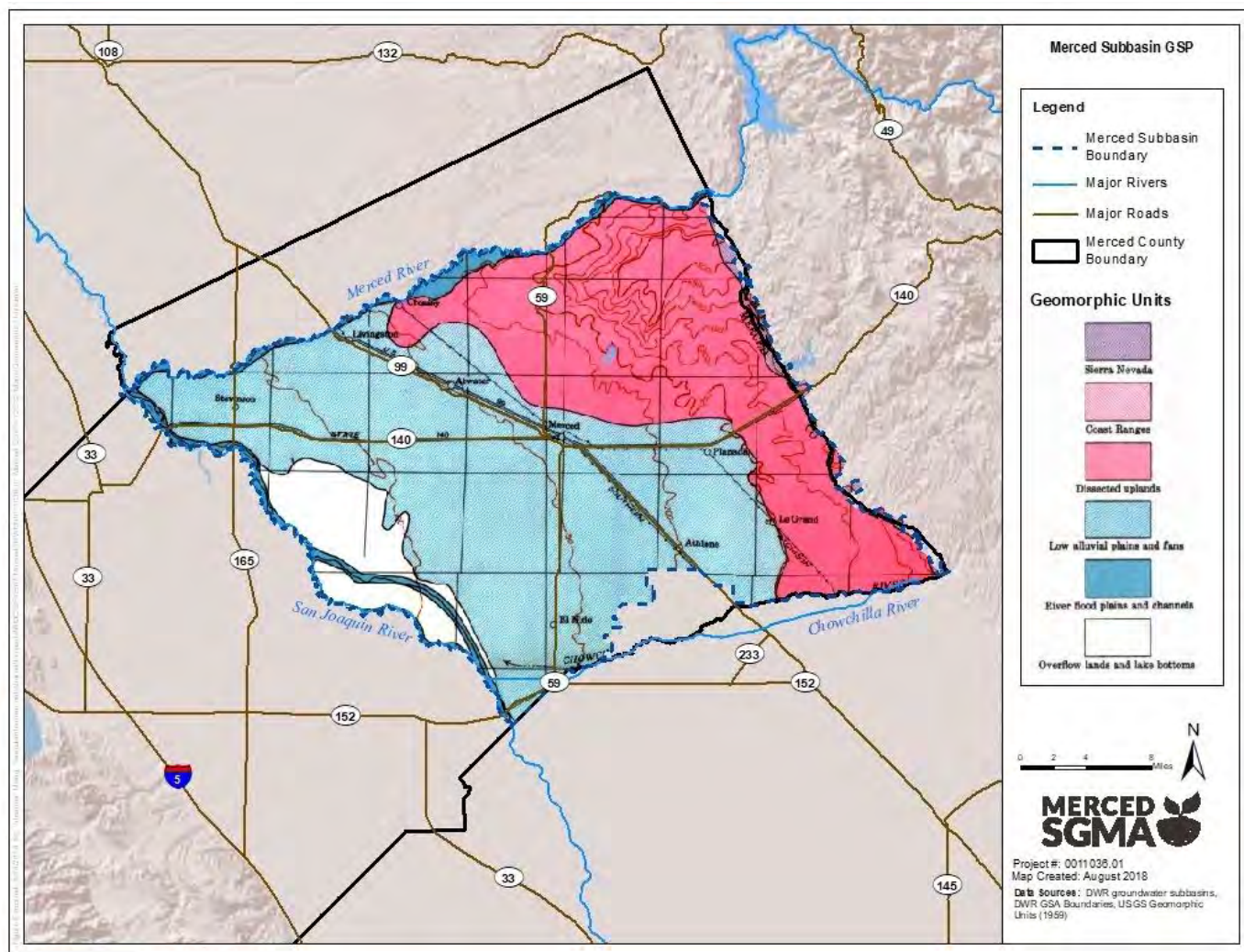
Figure 2-2: Geomorphic Units
