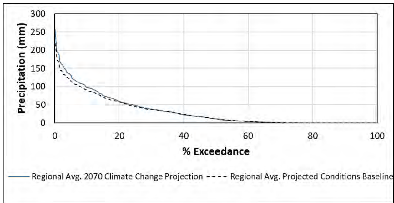
Figure 2-120: Perturbed Precipitation Exceedance Curve
