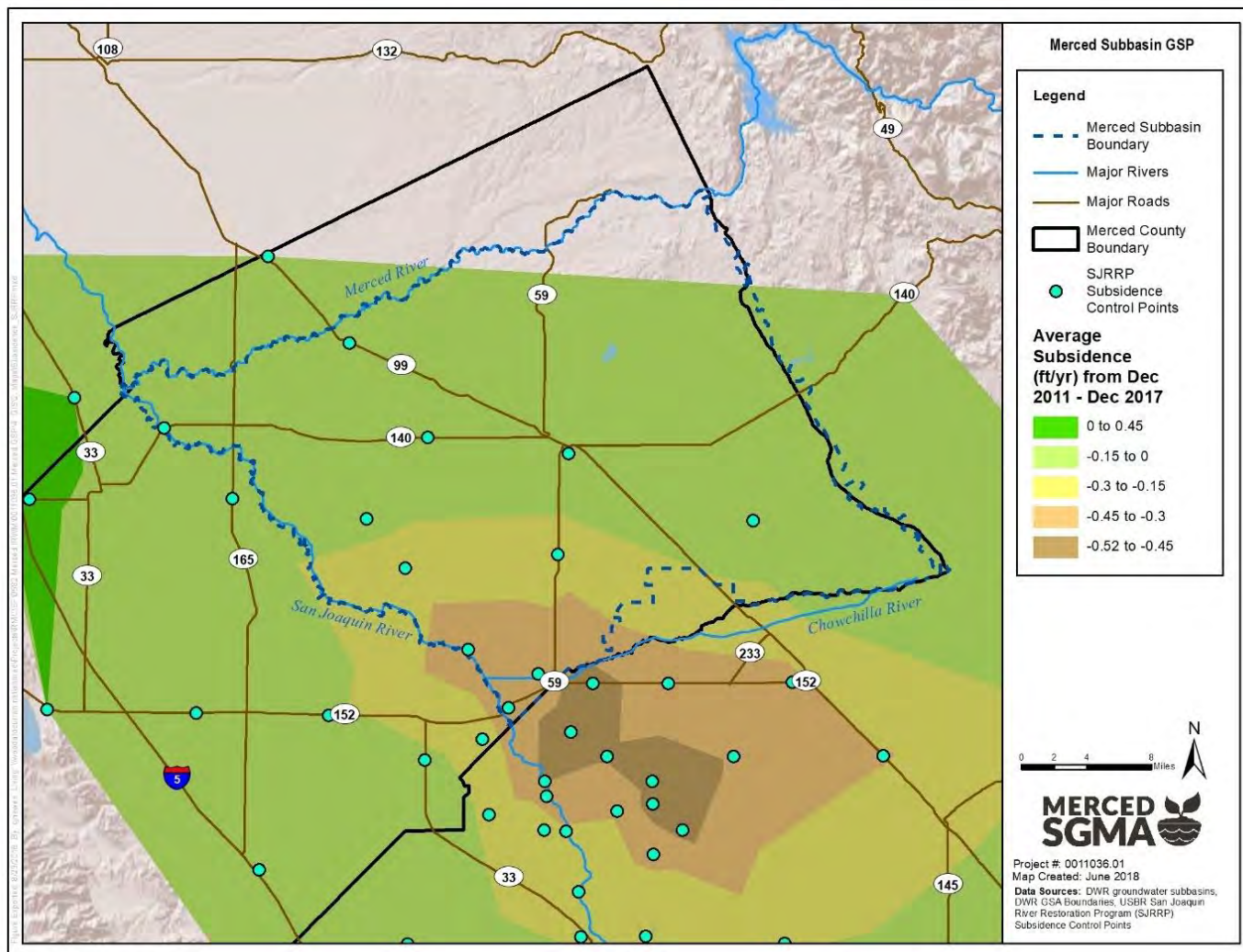
Figure 2-79: Average Land Subsidence December 2011 – December 2017
