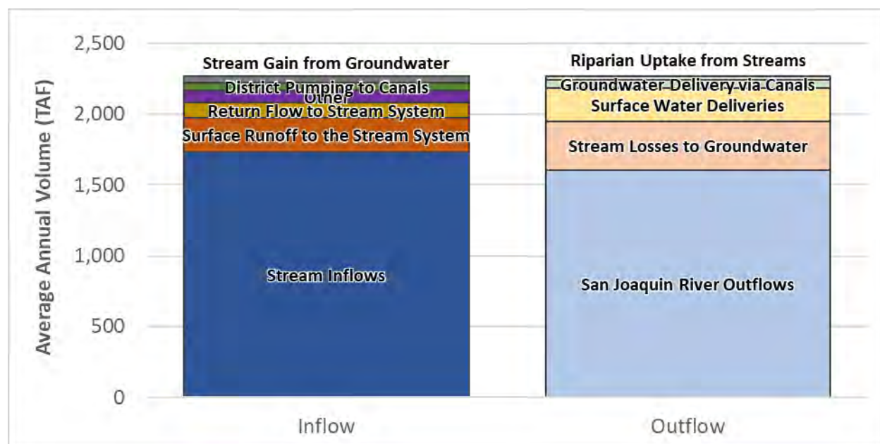
Figure 2-91: Historical Average Annual Water Budget – Stream and Canal Systems, Merced Subbasin
