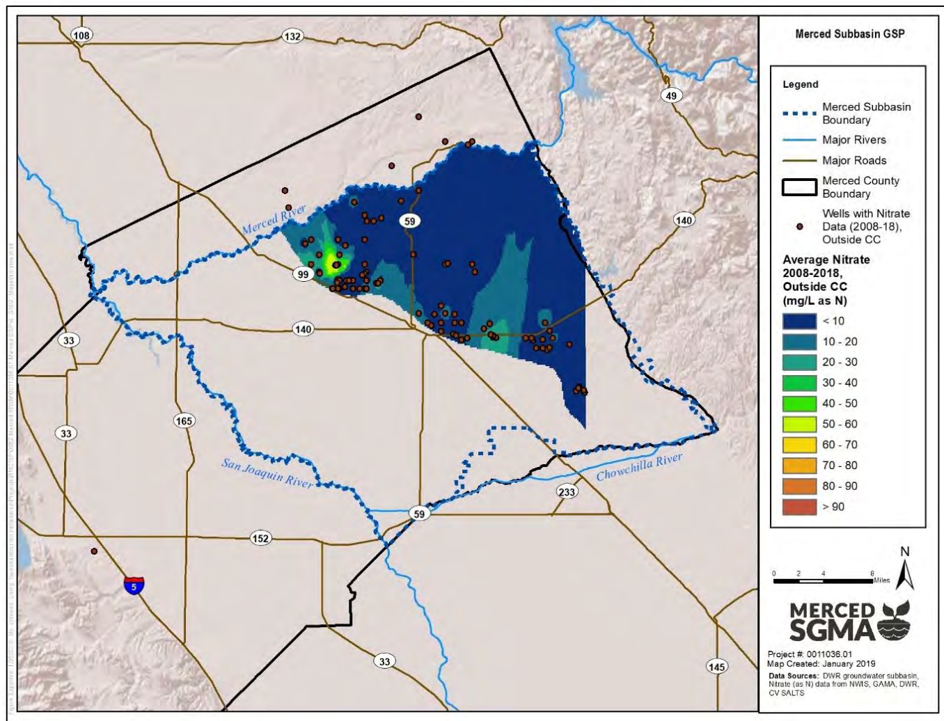
Figure 2-62: Average Nitrate (as N) Concentration 2008-2018, Outside Corcoran Clay
