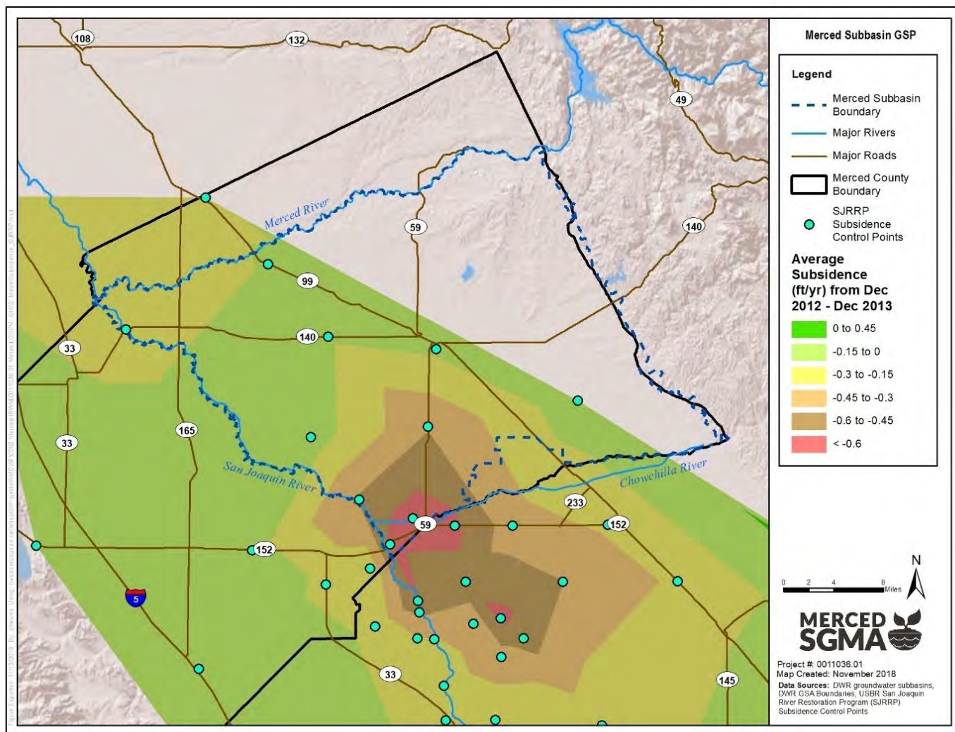
Figure 2-80: Land Subsidence December 2012 – December 2013
