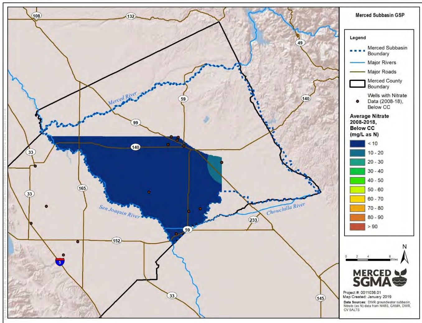
Figure 2-60: Average Nitrate (as N) Concentration 2008-2018, Below Corcoran Clay 1
