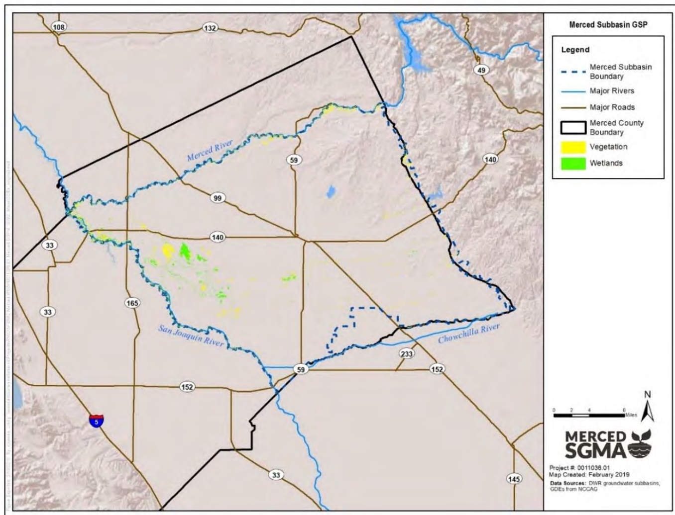
Figure 2-85: Natural Communities Commonly Associated with Groundwater (NCCAG)
