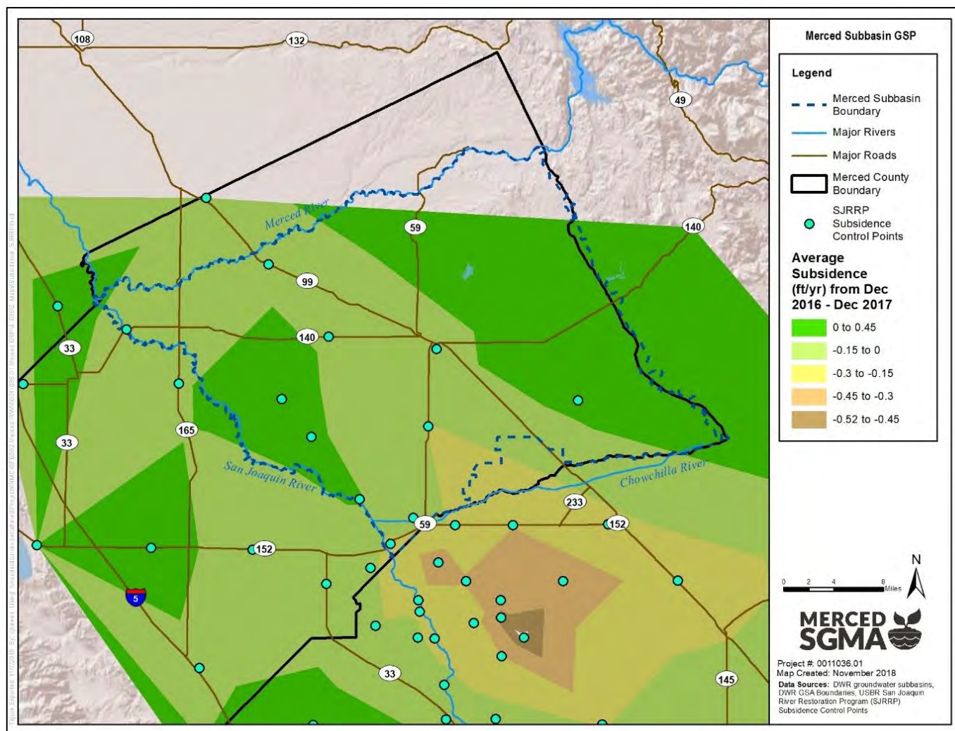
Figure 2-81: Land Subsidence December 2016 – December 2017
