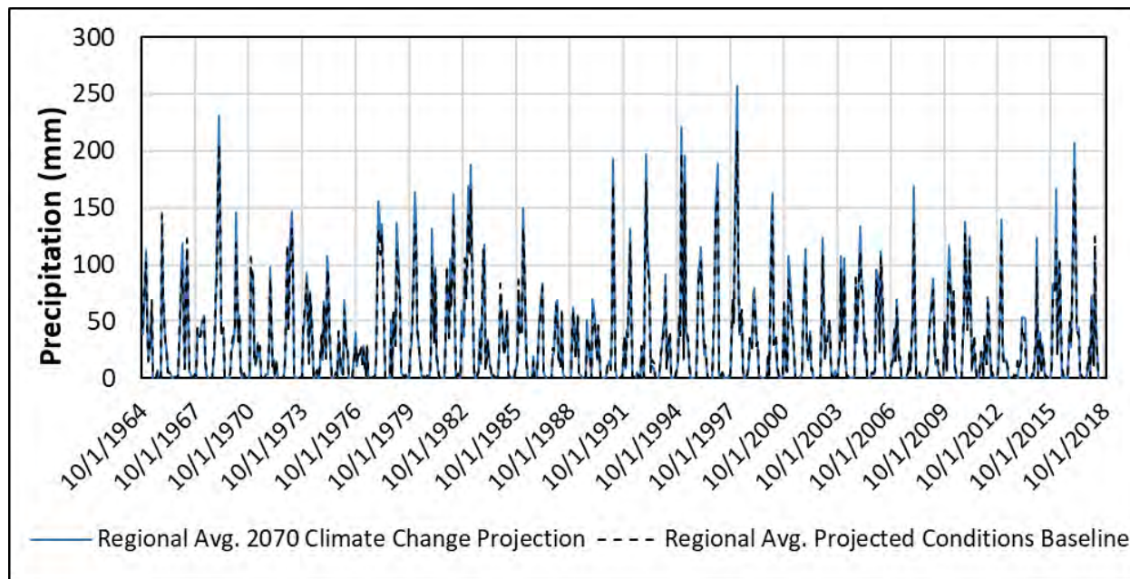
Figure 2-119: Perturbed Precipitation Under Climate Change
