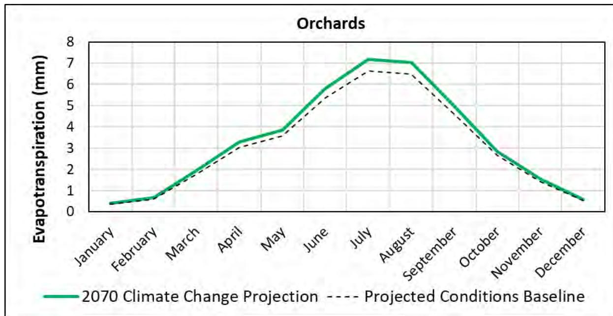
Figure 2-122: Monthly ET for Sample Crops
