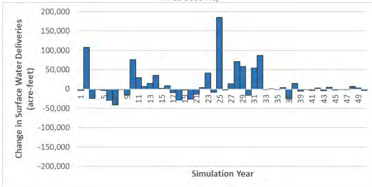
Figure 2-124: Simulated Changes in Surface Water Deliveries due to Climate Change (Scenario minus Baseline)
